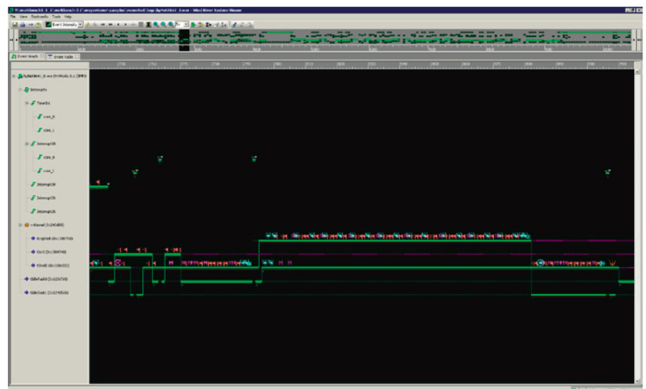
Figur 11 Systemvy i Wind River Workbench
